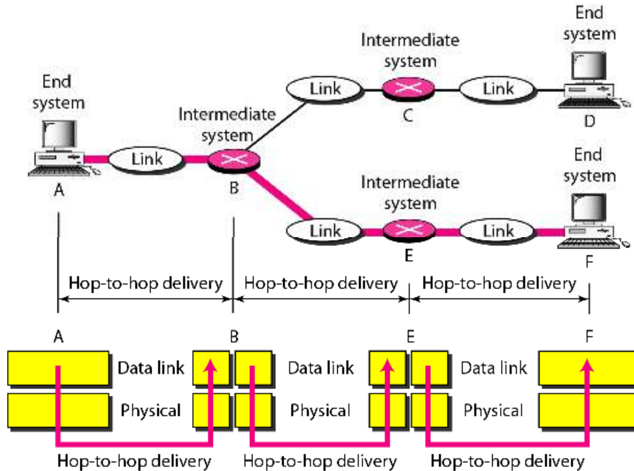
Figure 2.7 Hop-to-hop delivery
