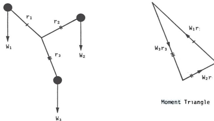
Figure 3: Moment triangle for static balance of three mass system
