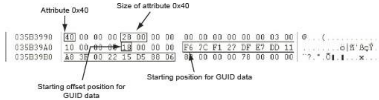
Figure 5-16 Attribute 0x40: Object_ID Courtesy of X-Ways AG, www.x-ways.net
