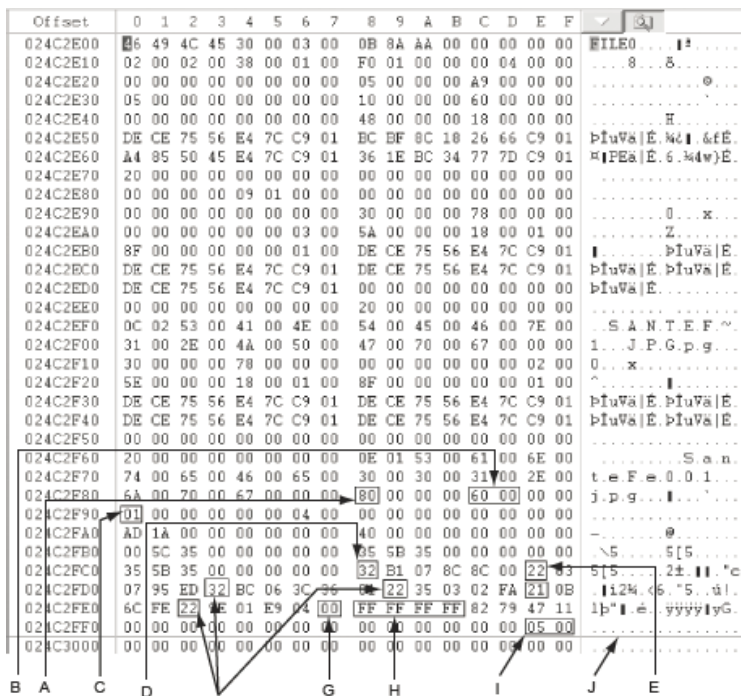
Figure 5-17 Attribute 0x80: Data for a resident file Courtesy of X-Ways AG, www.x-ways.net
