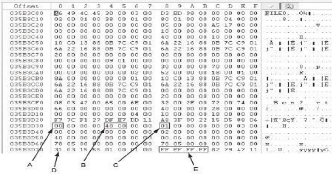
Figure 5-10 Resident file in an MFT record Courtesy of X-Ways AG, www.x-ways.net
