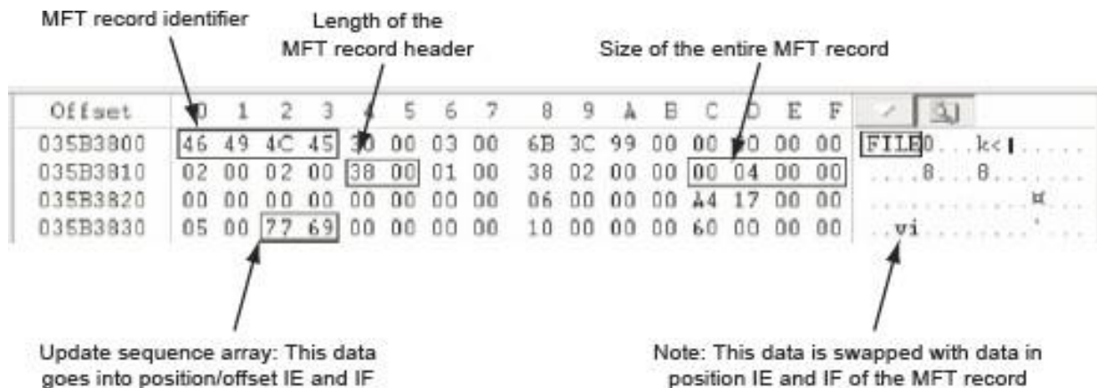
Figure 5-13 An MFT header Courtesy of X-Ways AG, www.x-ways.net
