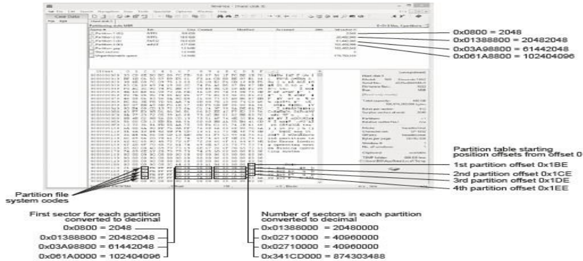
Figure 5-4 The partition table in a hexadecimal editor
