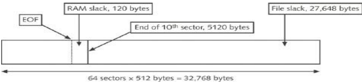
Figure 5-8 File slack space © 2015 Cengage Learning®
