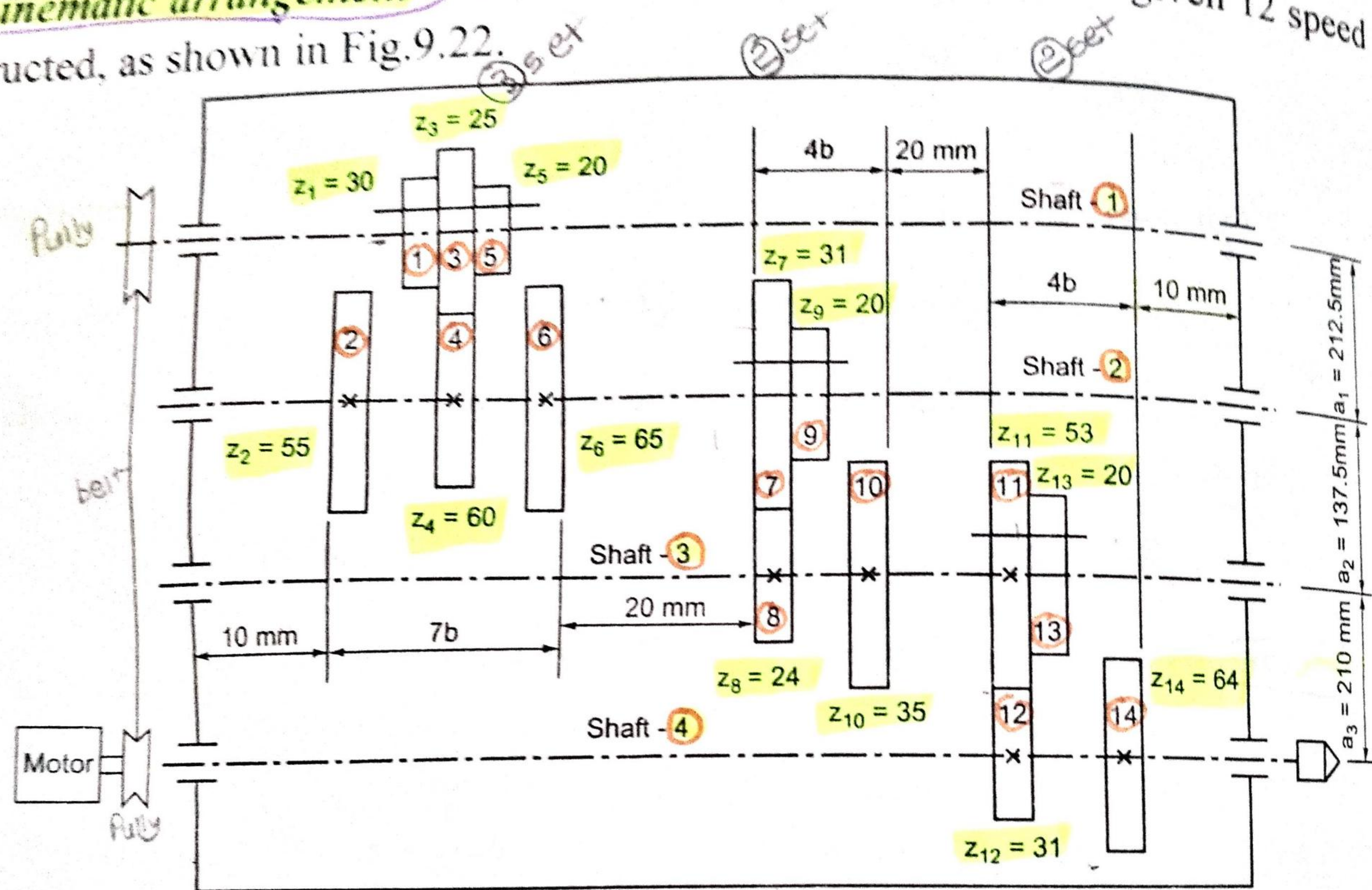
Fig. 9.22. Kinematic arrangement for 12 speed gear box
