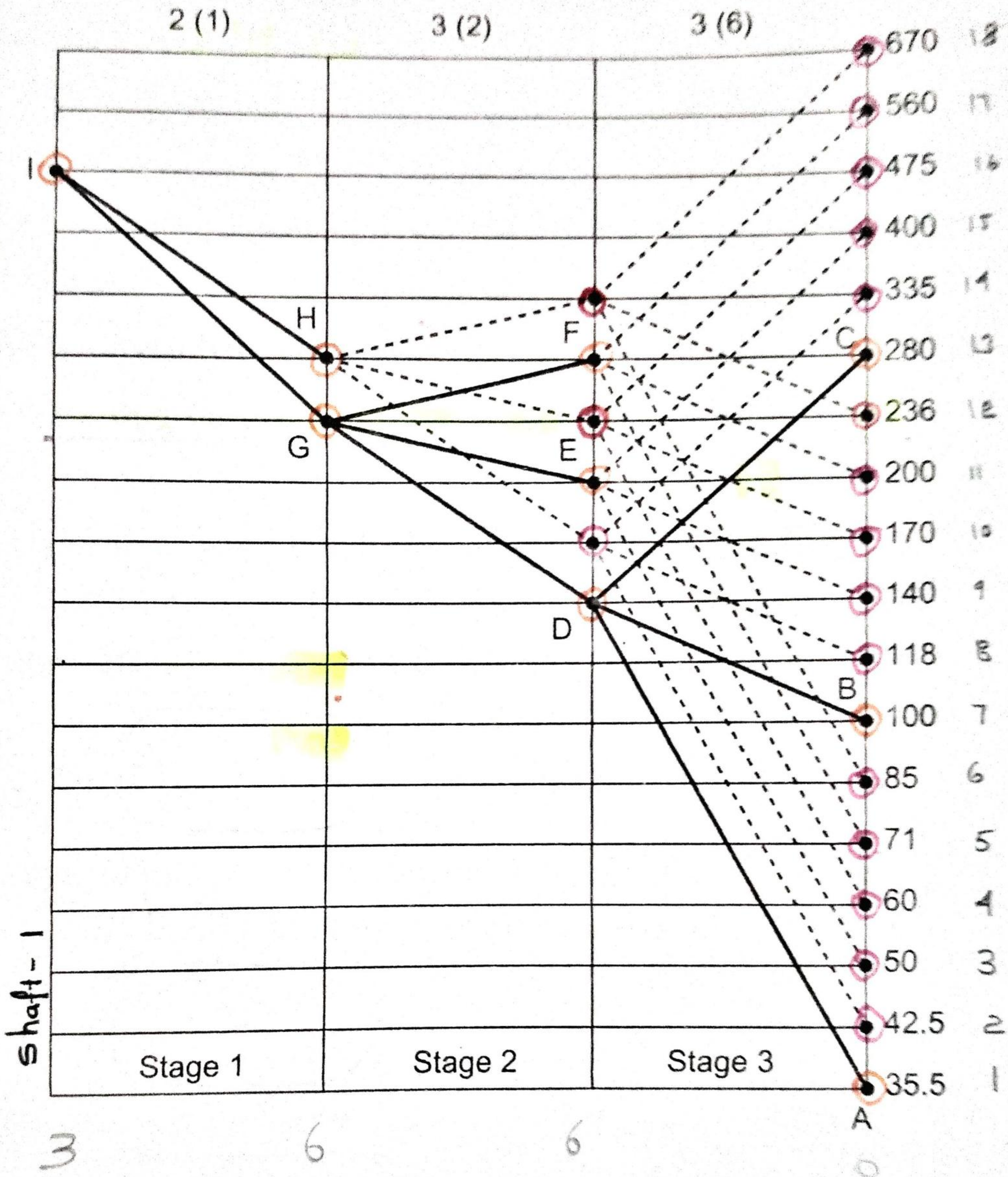
Fig. 9.23. Ray diagram for 18 speed gear box
