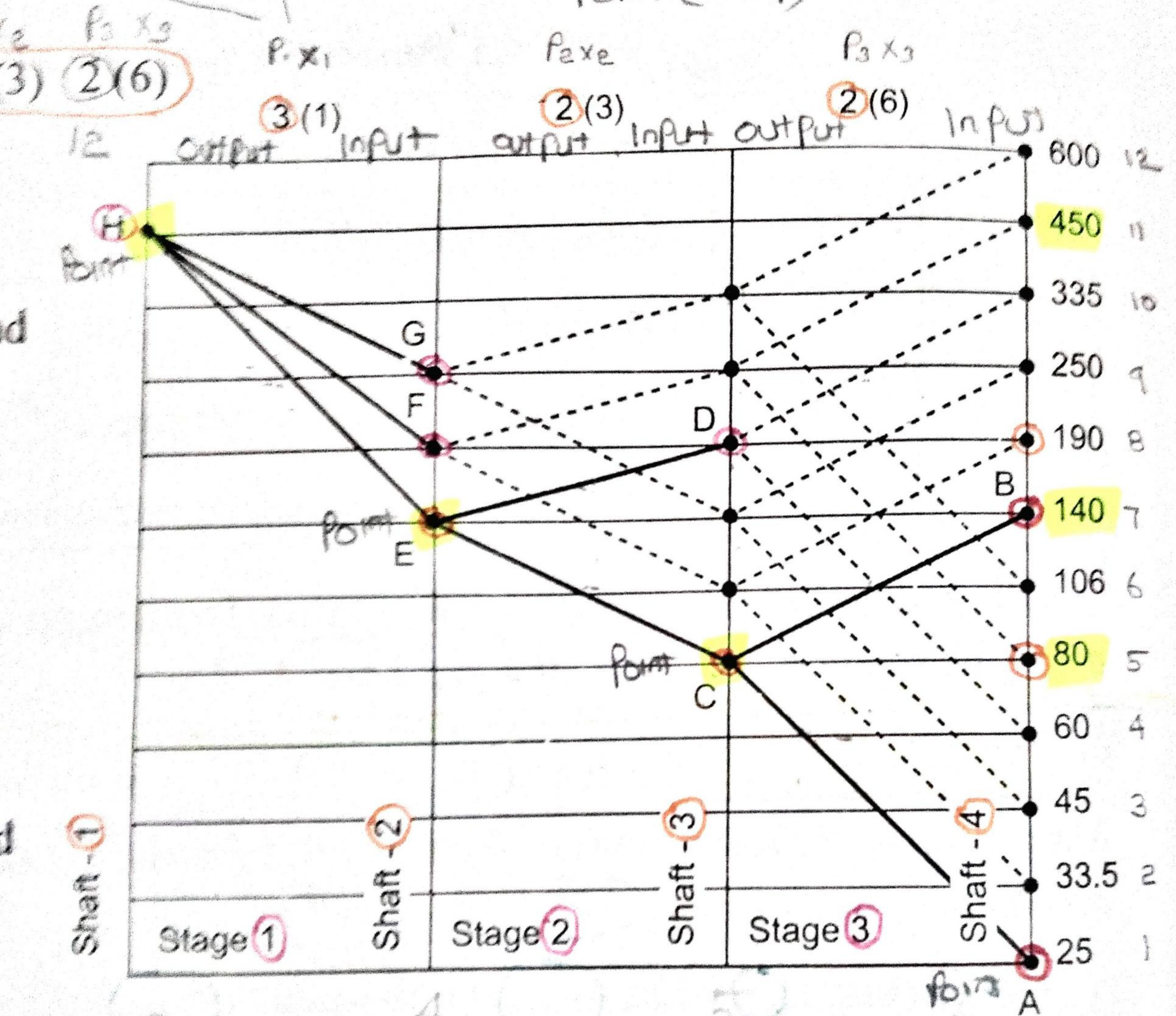
Fig. 9.21. Ray diagram for 12 speed gear box
